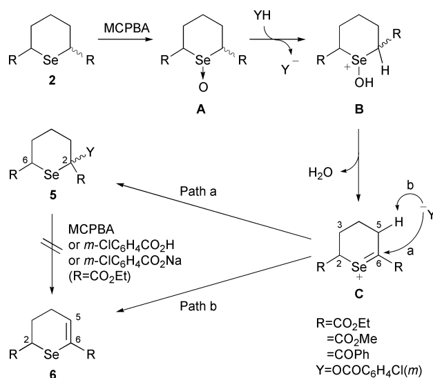
Scheme 2 Mechanism of the reactions of selenanes 2 with MCPBA.
