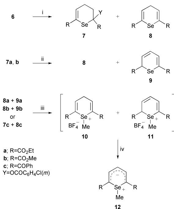
Scheme 3 Reagents and conditions: (i), MCPBA (1.1 equiv.), CH 2 Cl 2 ; (ii), PPSE, toluene, reflux, 20 h; (iii), MeI (6 equiv.), AgBF 4 (1.5 equiv.), CH 2 Cl 2 , 0 °C, 2 h; (iv), Et 3 N (3 equiv.), EtOH, 0 °C, 5 h.
