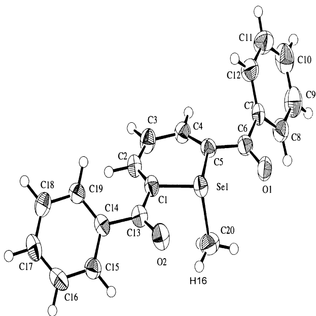
Fig. 3 ORTEP drawing for 12c .
