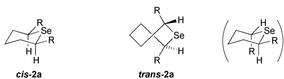
Fig. 1 Conformation of 2a .
