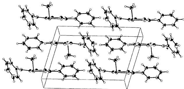
Fig. 4 Packing diagram for 12c .
