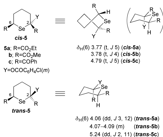
Fig. 2 Conformation of 5a–c .
